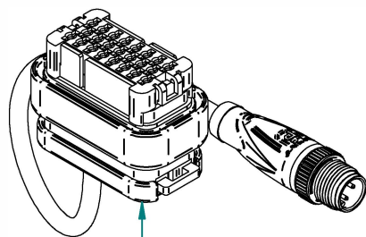
80733 Adapter cable AMPSEAL – M12
